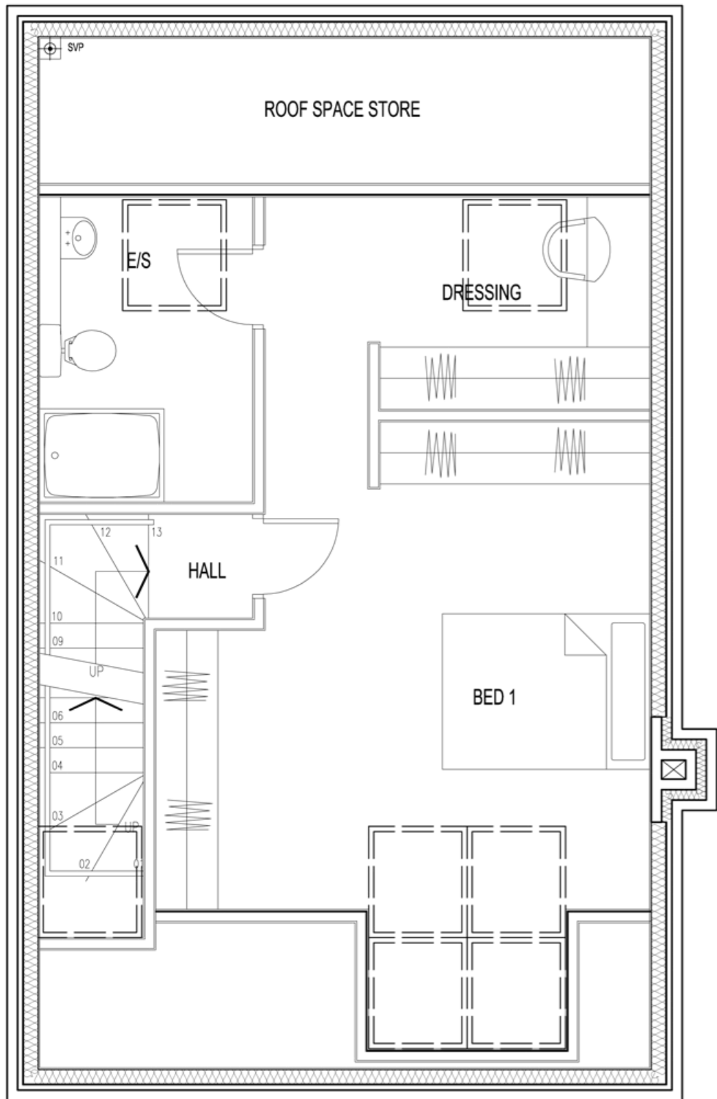
SECOND FLOOR PLAN SCALE 1:50
